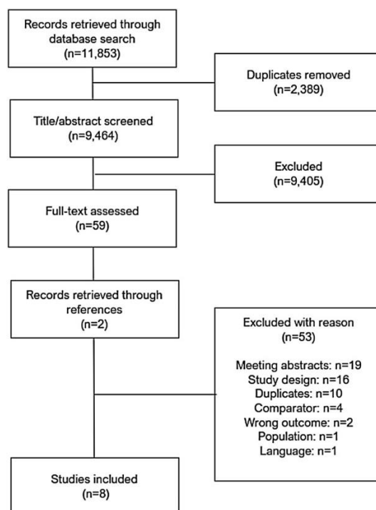
Figure 1. PRISMA flowchart
